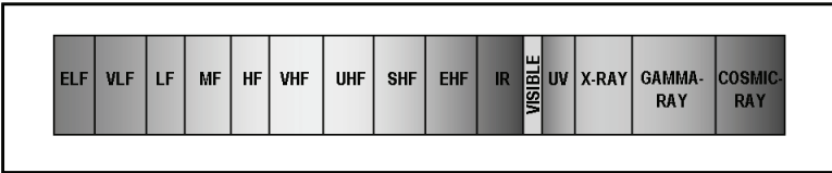
Figure A-1. The electromagnetic spectrum
